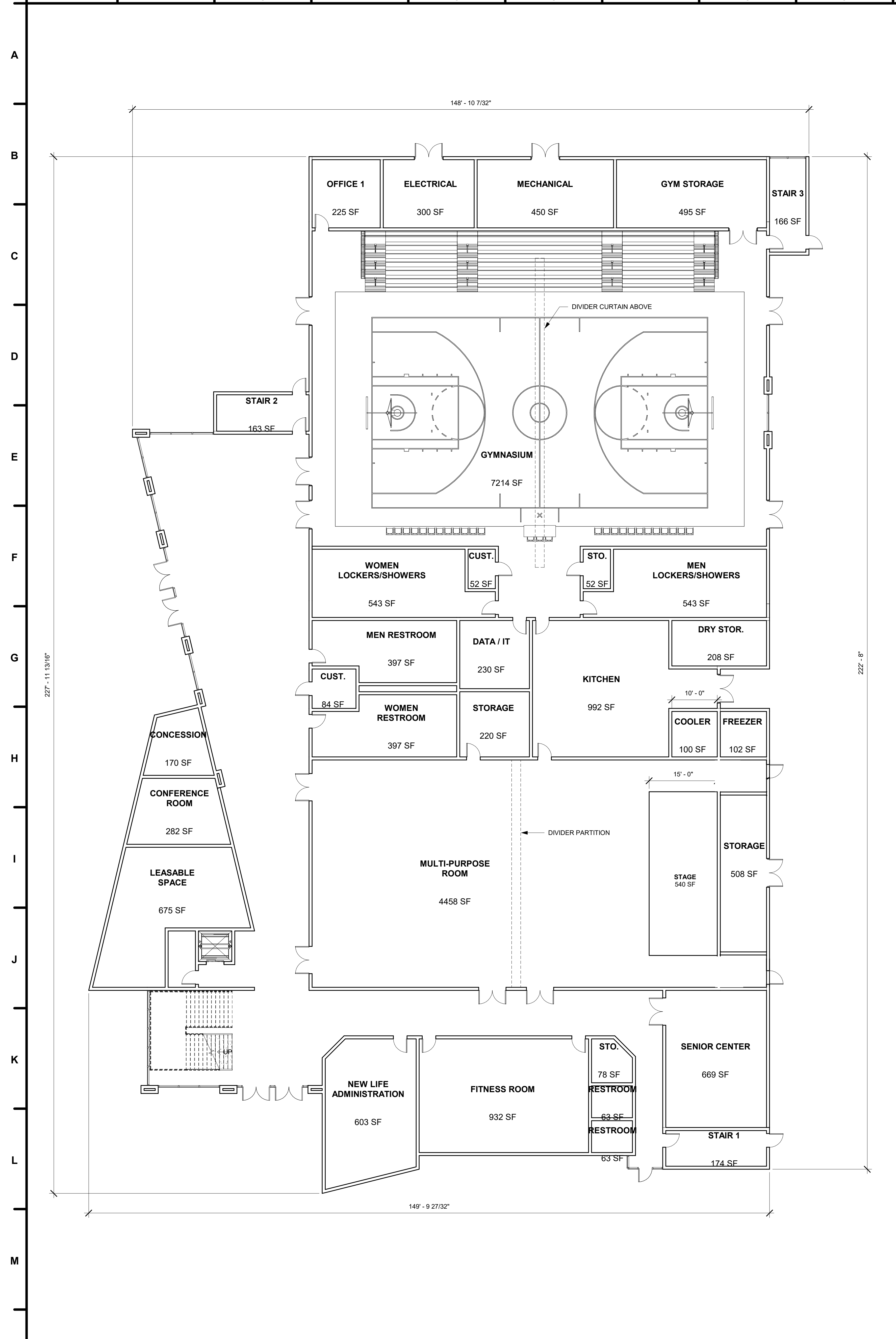
1 FIRST FLOOR 3/32" = 1'-0"
