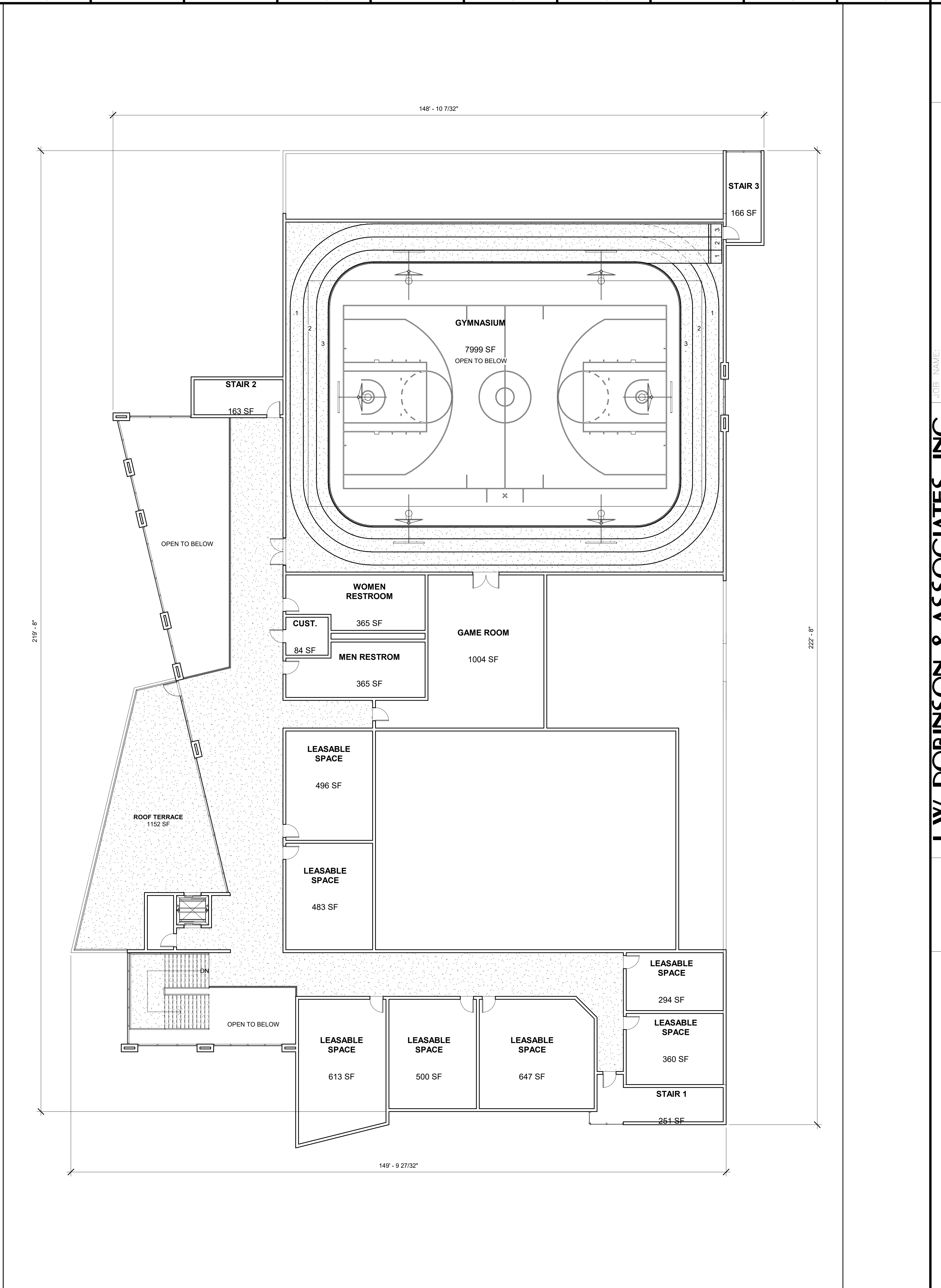
2 SECOND FLOOR 3/32" = 1'-0"
